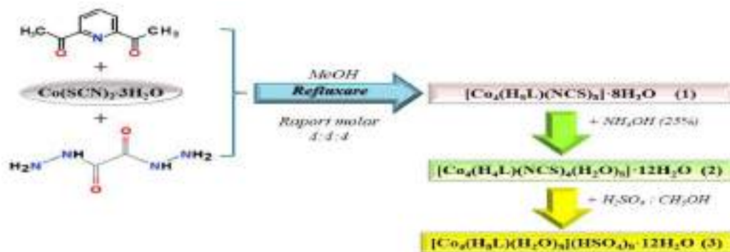
Figura 1. Schema de obținere a complexului macrociclic [\text{Co}_4(\text{H}_8\text{L})(\text{H}_2\text{O})_8](\text{HSO}_4)_8 \cdot 12\text{H}_2\text{O} ( 3 )
