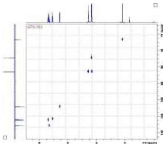
Figure 3. Spectrul ^1\text{H}/^{13}\text{C} HSQC RMN al compusului 4
