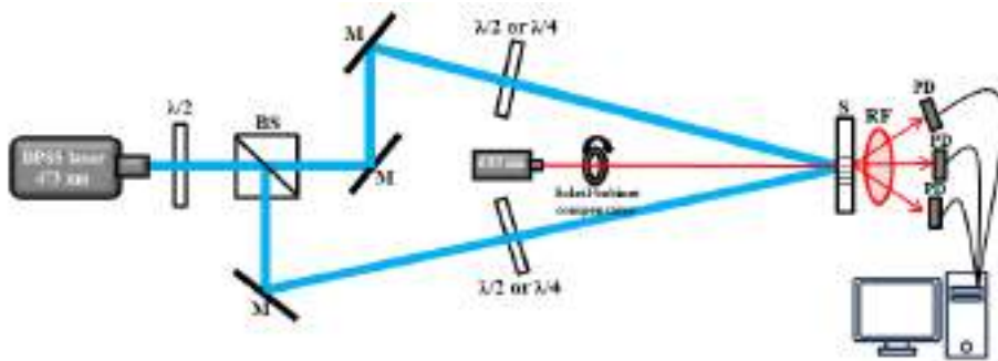
Figure 3. Optical Setup for Polarization Holographic Recording
