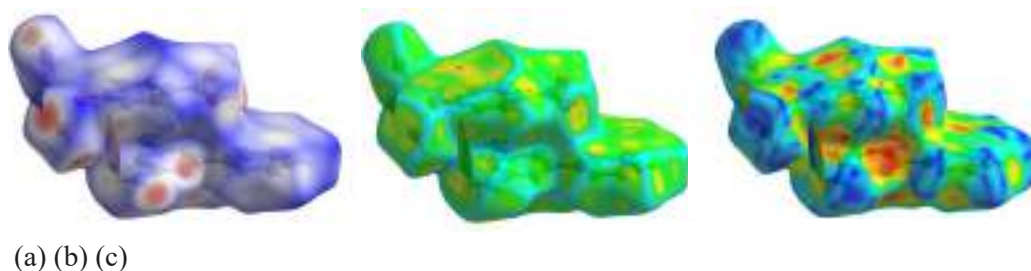
Figure 3. 3D Hirshfeld surfaces of the title cocrystal mapped with a) d norm (min: -0.7668, mean: 0.3843, max: 1.1187); b) Curvedness (min: -3.4198, mean: -0.9583, max: 0.8936); c) Shape index (min: -0.9938, mean: 0.2234, max: 0.9972)
